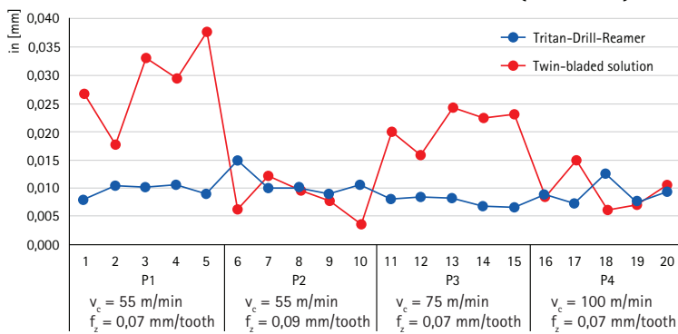
Diameter deviation over the tools entire diameter (42CrMoS4)
